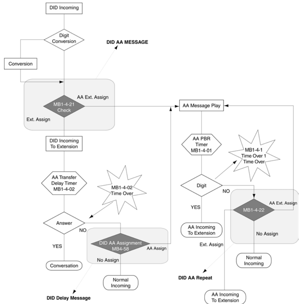
Figure A8-1: Direct Inward Dialling Operation
